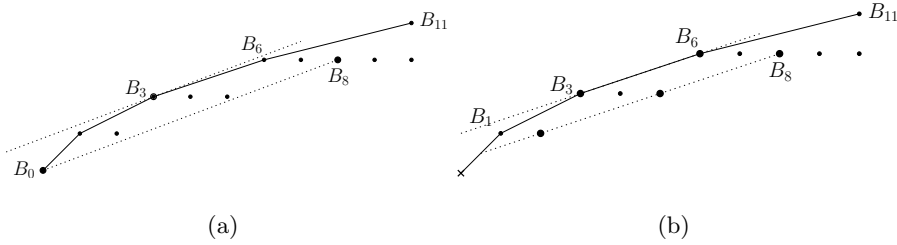
Fig. 7. B_0 is removed from the segment (B_0B_8) that is maximal at the front. Since B_3 is a vertex of (\overline{B_0B_{11}}) by hypothesis, B_6 is the next vertex of (\overline{B_0B_{11}}) .
