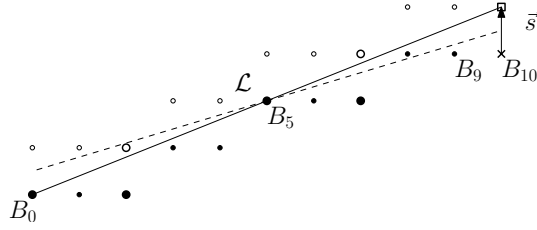
Fig. 6. B_{10} is weakly exterior to \mathcal{D}(2, 5, 0) . The first and last leaning points on the left of (B_0B_9) ( B_0 and B_5 ) and B_{10} + \vec{s} are collinear. Since B_0 is a vertex of (\overline{B_0B_{10}}) by hypothesis, B_5 is the next vertex of (\overline{B_0B_{10}}) .
