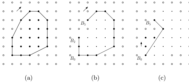
Fig. 3. In (a), the digital object depicted with black points is not convex because its convex hull contains one background point. In (b), the part (B_5 B_2) is convex because there is no digital point between \overline{(B_5 B_2)} and (B_5 B_2) . Conversely, in (c), the part (B_0 B_5) is concave because there is no digital point between \underline{(B_0 B_5)} and (B_0 B_5) .
